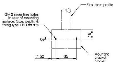
MOUNTING HOLES Dimensions in mm
