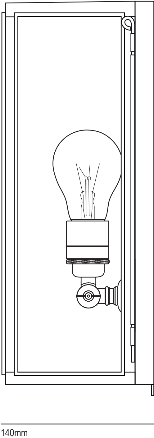
Side View
