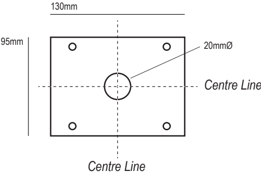
Rear Cable Entry Fixing Bracket
